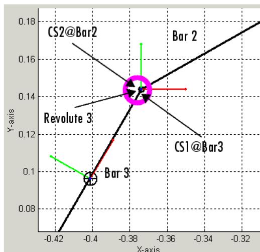
Assembled Revolute Joint in the Four Bar Mechanism
