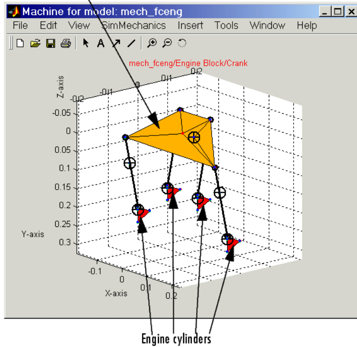
Four Cylinder Engine Example: Engine Crank Convex Hull (Yellow)
