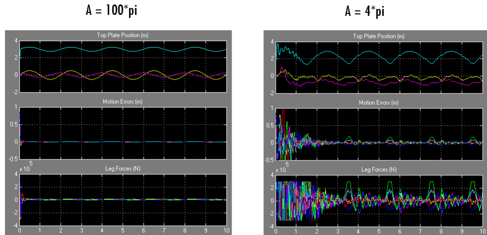
Stewart Platform Motion and Forces with PID Controller (Filtered Derivative)
